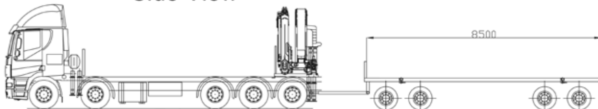
Side View
